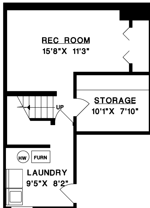
LOWER FLOOR
