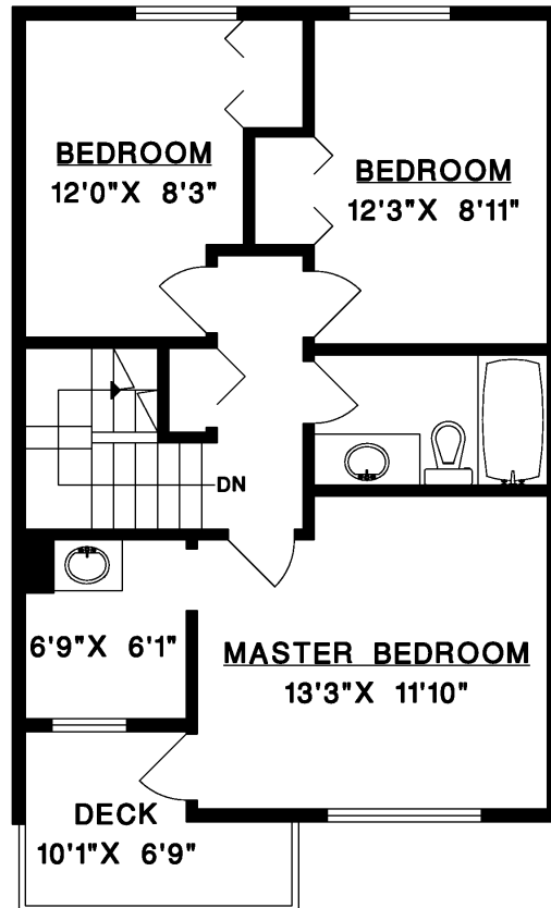
UPPER FLOOR
