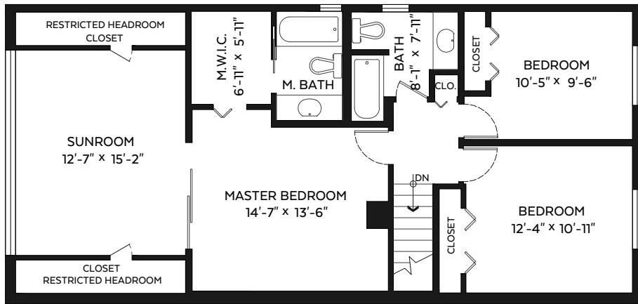
Upper Floor Plan Floor Area: 961 sq.ft.
